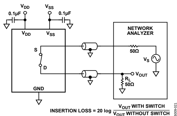
Figure 22. Bandwidth
